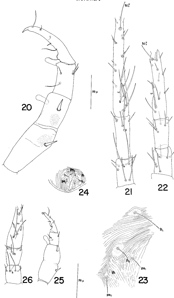
Figs. 20-26. Dactyloscirus smileyi sp. nov. (20) Right palpus, female; (21) genu, tibia and tarsus of leg I, female; (22) genu, tibia and tarsus of leg II, female; (23) integrated H and PS tergites showing h_{1-2} and ps_{1-2} setae, cupule ih , female; (24) pseudanal plate with h_2 , ps_{1-2} setae and cupule ih , larva; (25) right palpus, larva; (26) leg I, larva.
