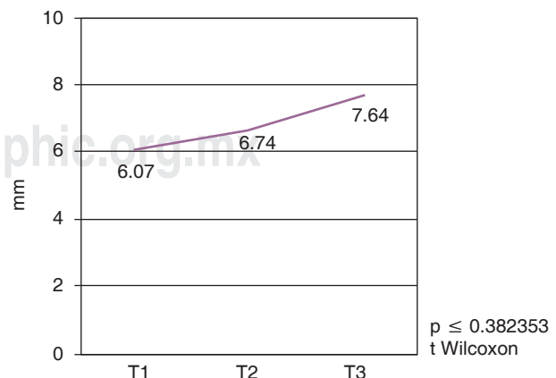
Figure 7. Difference between means at T1, T2, T3. \bar{X} Columella.
