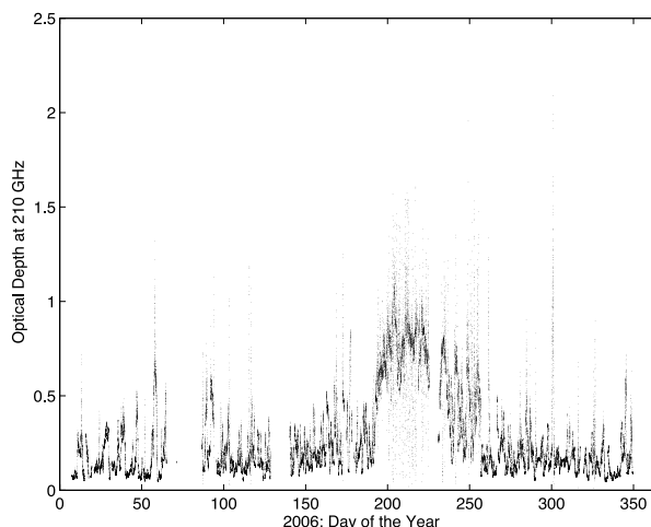
Fig. 5. SY2006, 210 GHz optical depth time series. The time resolution of the tipper measurements is 6 minutes.
