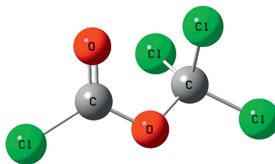
Figure 2 Representation of diposgene.
