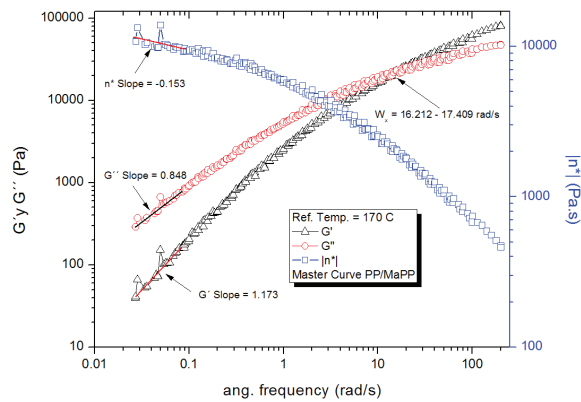
Figure 5. PP/MaPP master curve from the frequency sweeps: 0.1 to 200 and 200 to 0.1 rad/s at 170, 190 and 210°C. Reference temperature of 170°C
