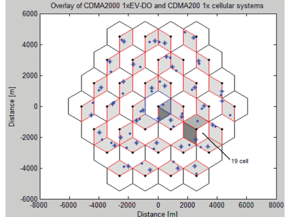
Figure 1. Macrocell CDMA1xEV-DO system scenario
