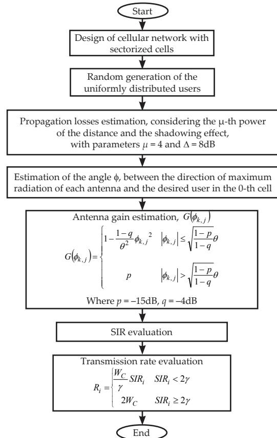
Figure 2. Dataflow of the Monte Carlo simulation
