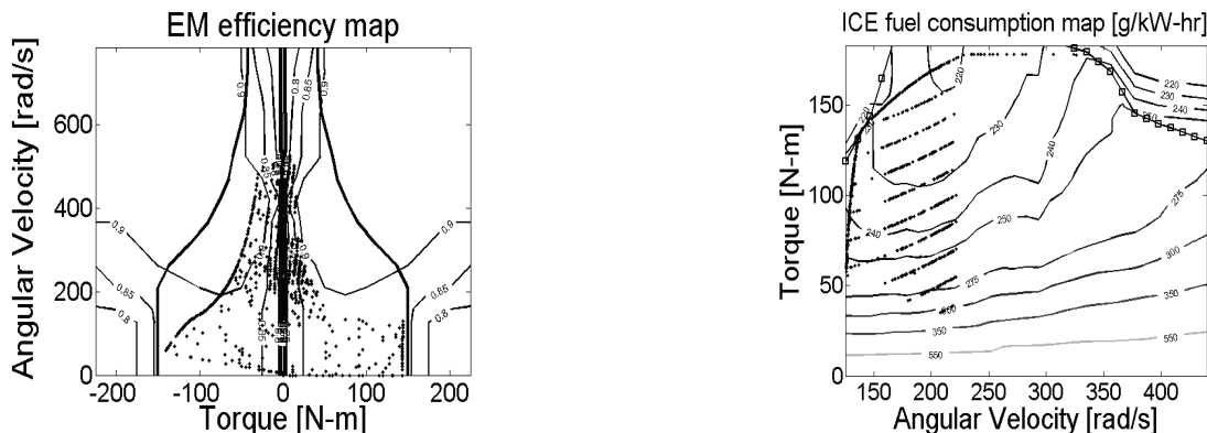
Figure 8. Efficiency and fuel consumption maps
